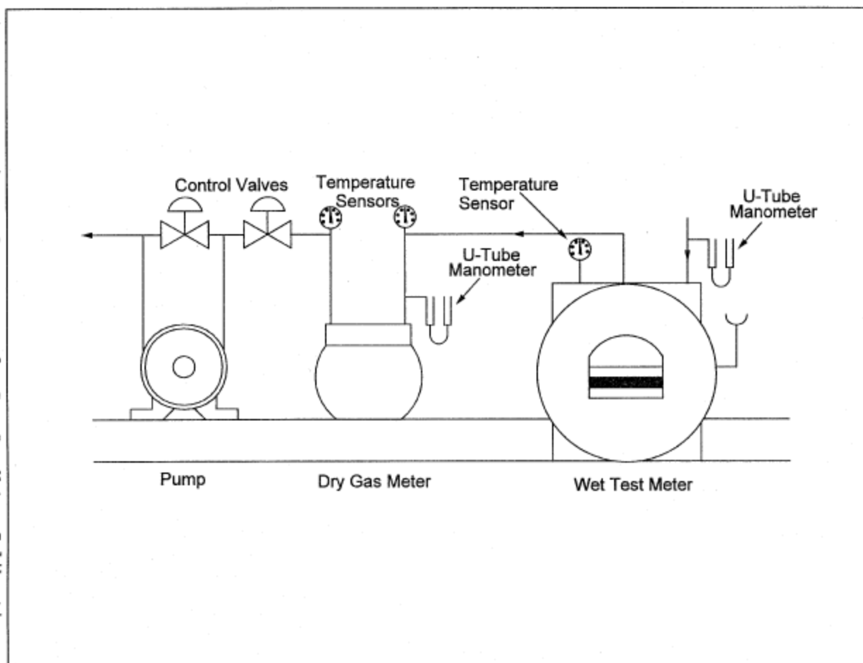
Figure 5-7. Equipment Arrangement for Dry Gas Meter Calibration.
