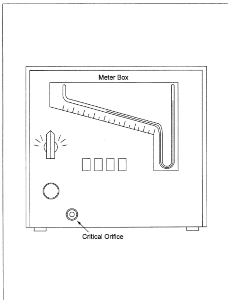
Figure 5-10. Apparatus Setup.
