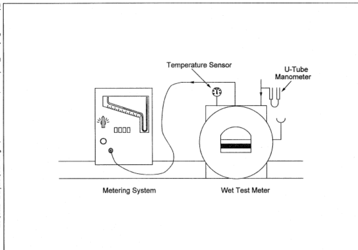
Figure 5-4. Equipment arrangement for metering system calibration.
